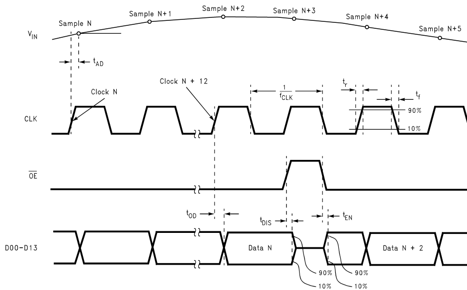
Output Timing
