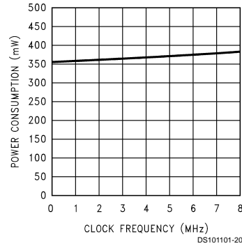
Power Consumption vs f_{CLK}
