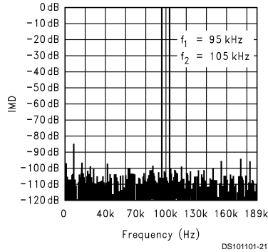
IMD Response
