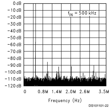
Spectral Response
